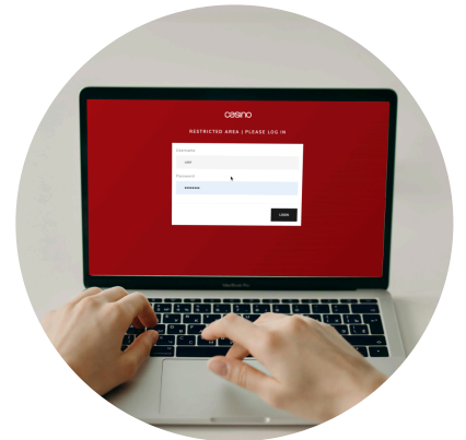
Backend Software
